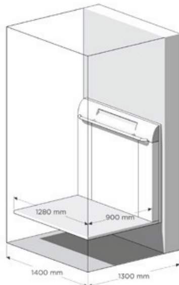
900 x 1280
