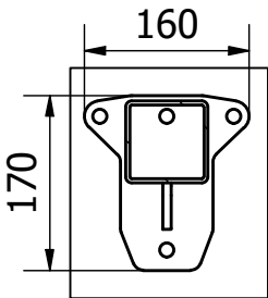
Typical stanchion
