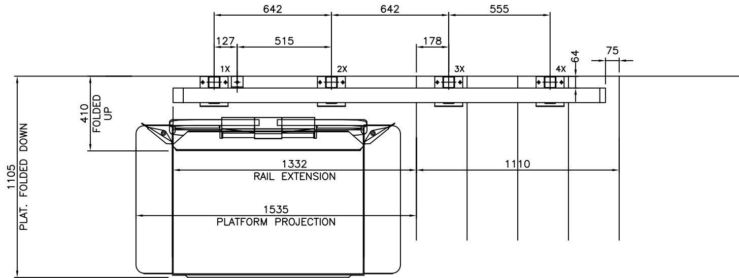
PLAN TOWER MOUNT UNIT
